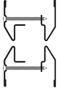
LT-B4 1 1/16" Glazing Pocket for 7/8" to 1" Glass
