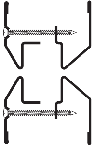
LT-B3 13/16" Glazing Pocket for 5/8" to 3/4" Glass
