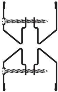
LT-B1 3/8" Glazing Pocket for 1/4" Glass
