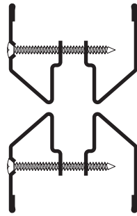
LT-B2 9/16" Glazing Pocket for 3/8" to 1/2" Glass
