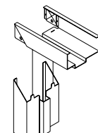
Corner Connection
