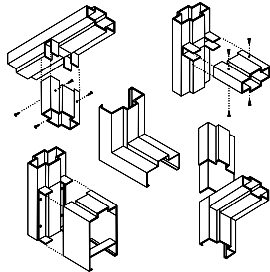
Section Details of Typical Field Splice Connections
