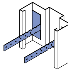
L Strap Anchor (Optional)
