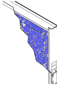
Polystyrene Core
