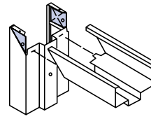
MH Corner Connection
