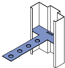
"T" Anchor
