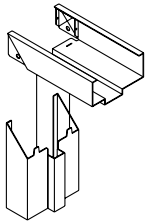
ME Corner Connection
