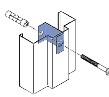
Prepared Opening Anchor
