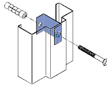
Prepared Opening Anchor
