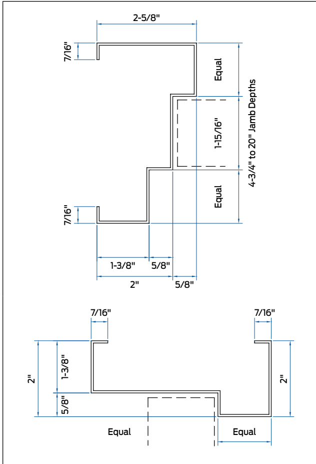
1-3/8" Face (standard)
