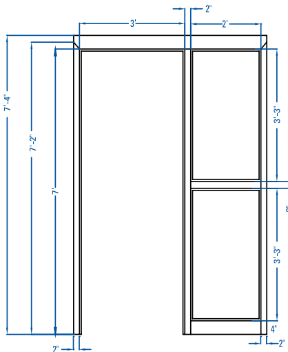
Overall 5674 Elevation with Side light
